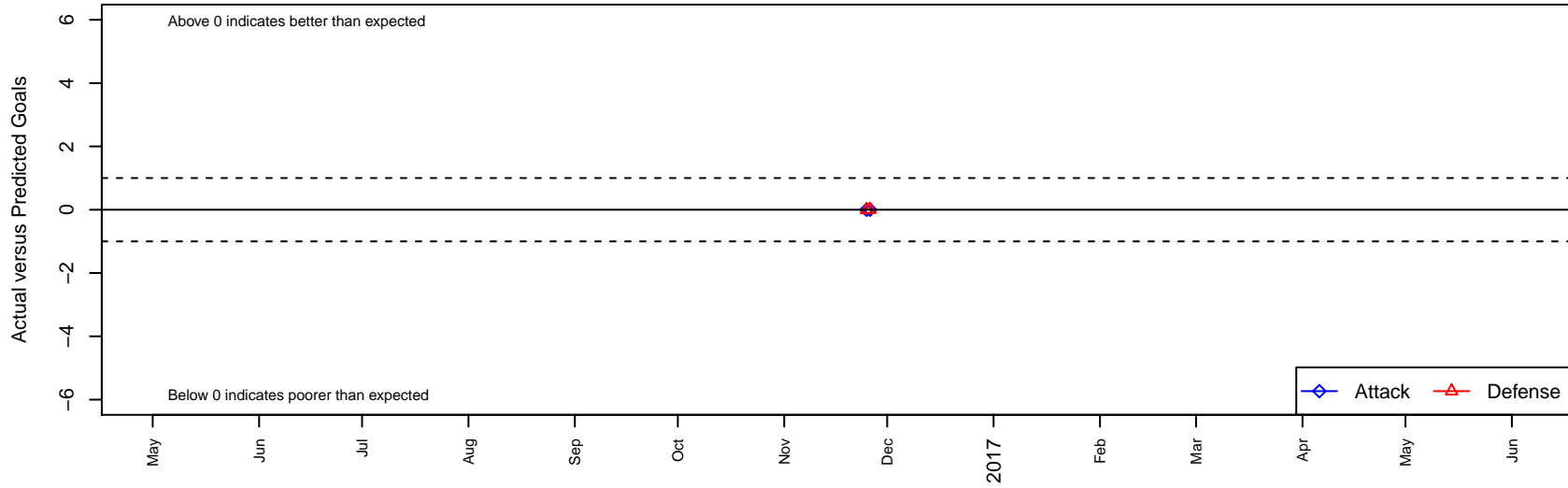
San Francisco Academy Elite B02 Dots are actual minus expected GF (blue circles) and GA (red triangles). Blue line is smoothed change in attack strength. Red is smoothed change in defense strength.
